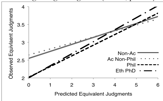
Figure 2: Linear regression trendlines for the number of scenario pairs rated as equivalent as a function of number of scenario pairs presented in an order favoring equivalent judgment. Greater slope indicates stronger equivalency order effects on moral judgment.
